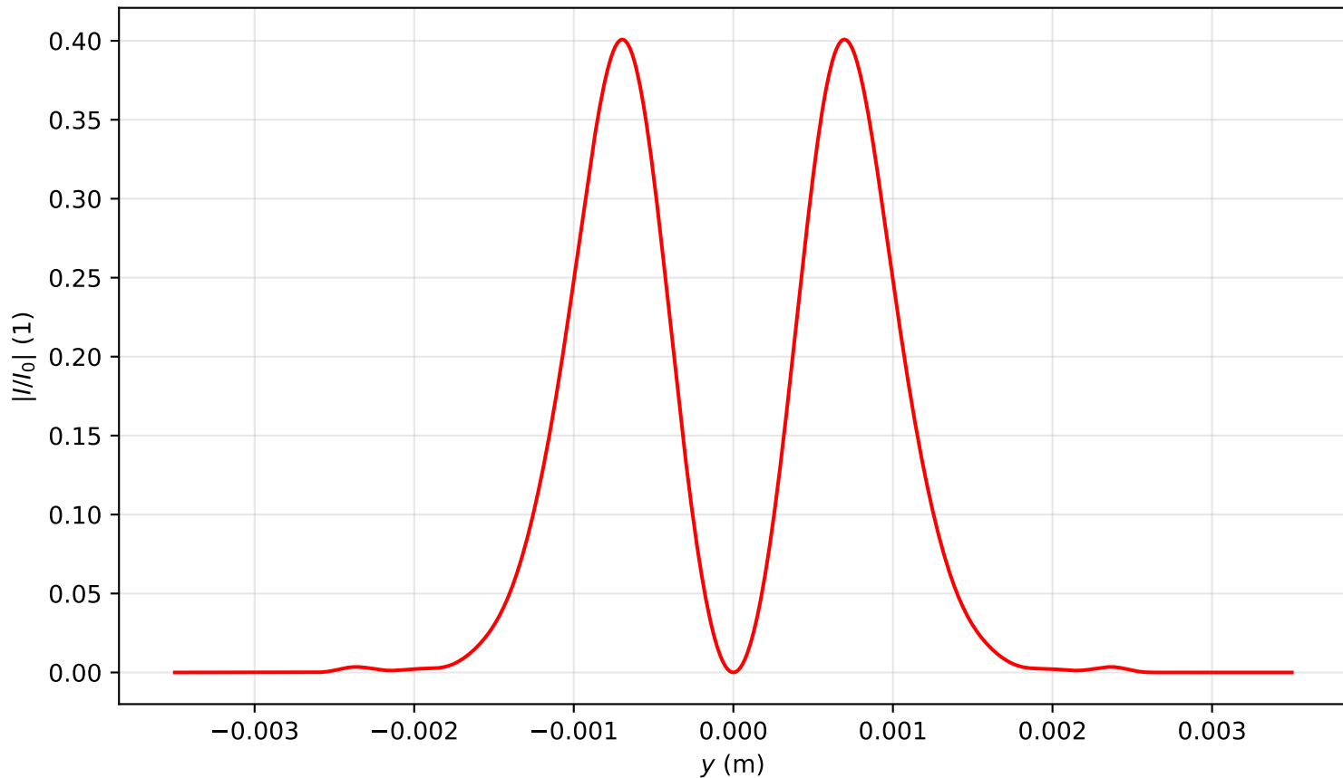
Intensity profile I(x=0, y, z=2.468)/I_0 , P_{in}=3.0P_{cr} , artificial time
